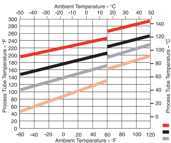
TPE1 - ONE 1/2" (12mm) PROCESS LINE WITH HIGH TEMPERATURE TRACER
